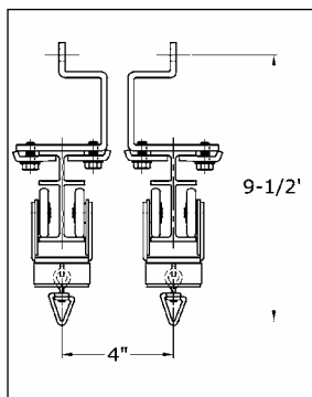
Cross Section of 500 Suspended
