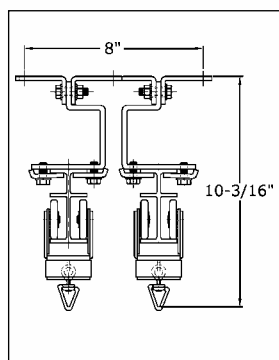
Cross Section of 500 Ceiling Mount
