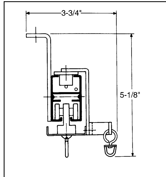
Cross Section of 114 Track
